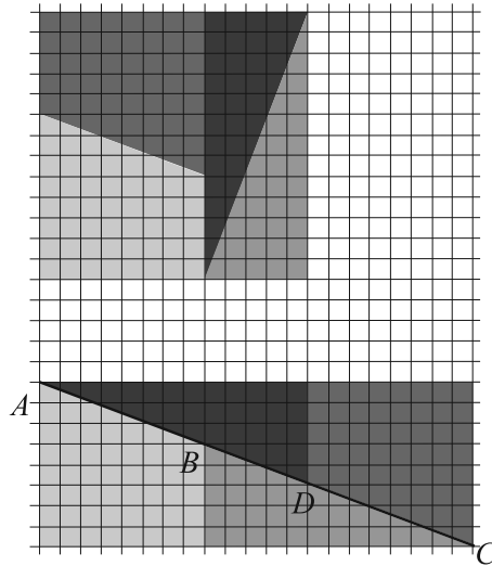
Рис. 1.1 – f(7)^2 и f(6) \times f(8)
